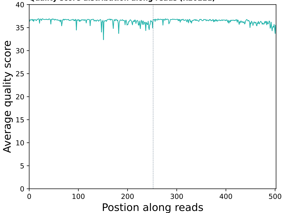
Quality score distribution along reads (R20221)
